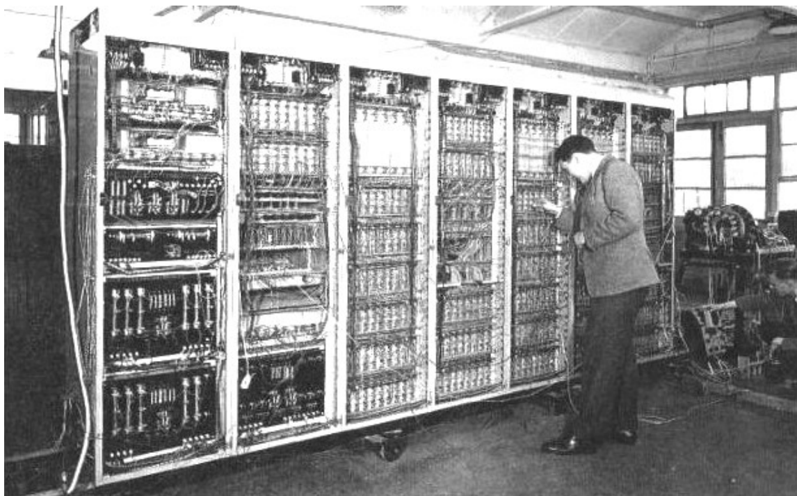
Part of the WREDAC computing equipment under test
